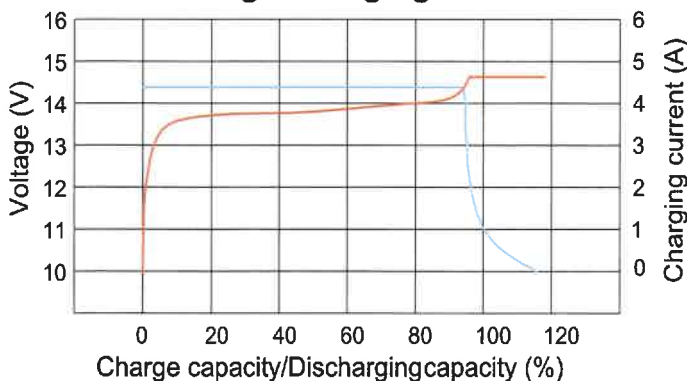
Constant voltage charging characteristics
