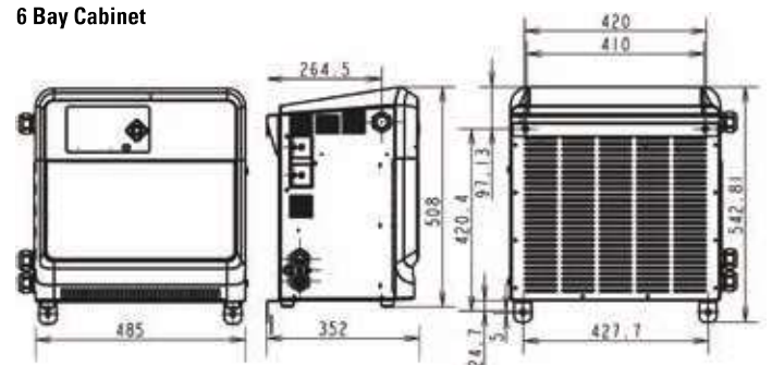
6 Bay Cabinet
