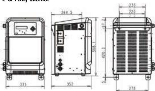
2 & 4 Bay Cabinet
