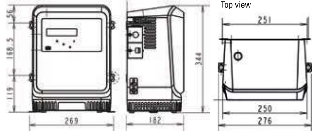
3 Bay Cabinet
